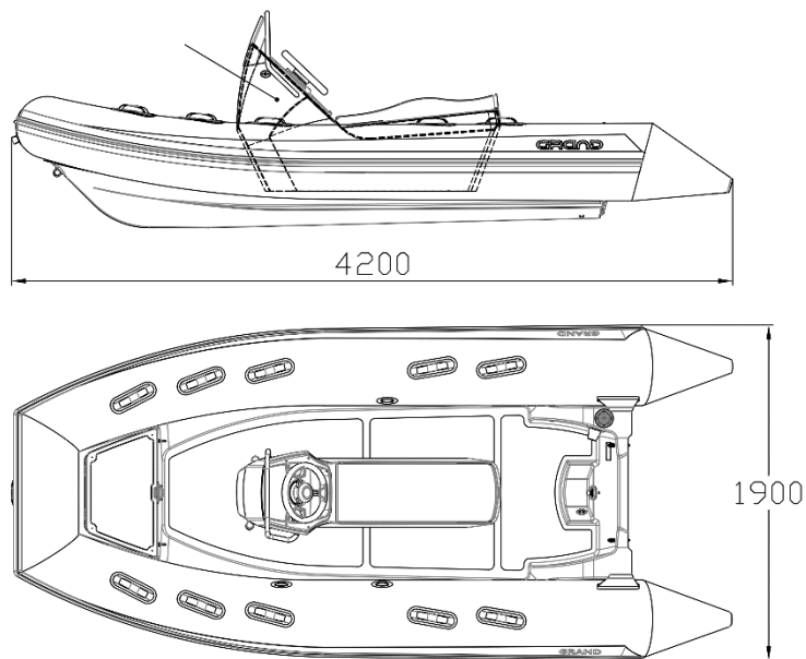
Fig. 52. General view of a boat S420NS.
