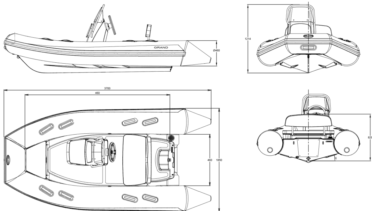
Fig. 46. General view of a boat S370NL.
