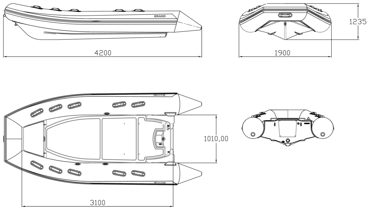
Fig. 51. General view of a boat S420N.
