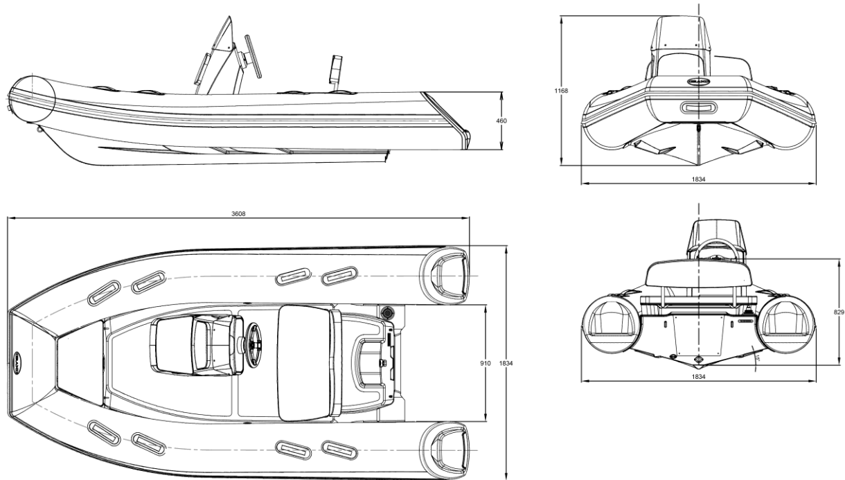
Fig. 47. General view of a boat S370NLF.
