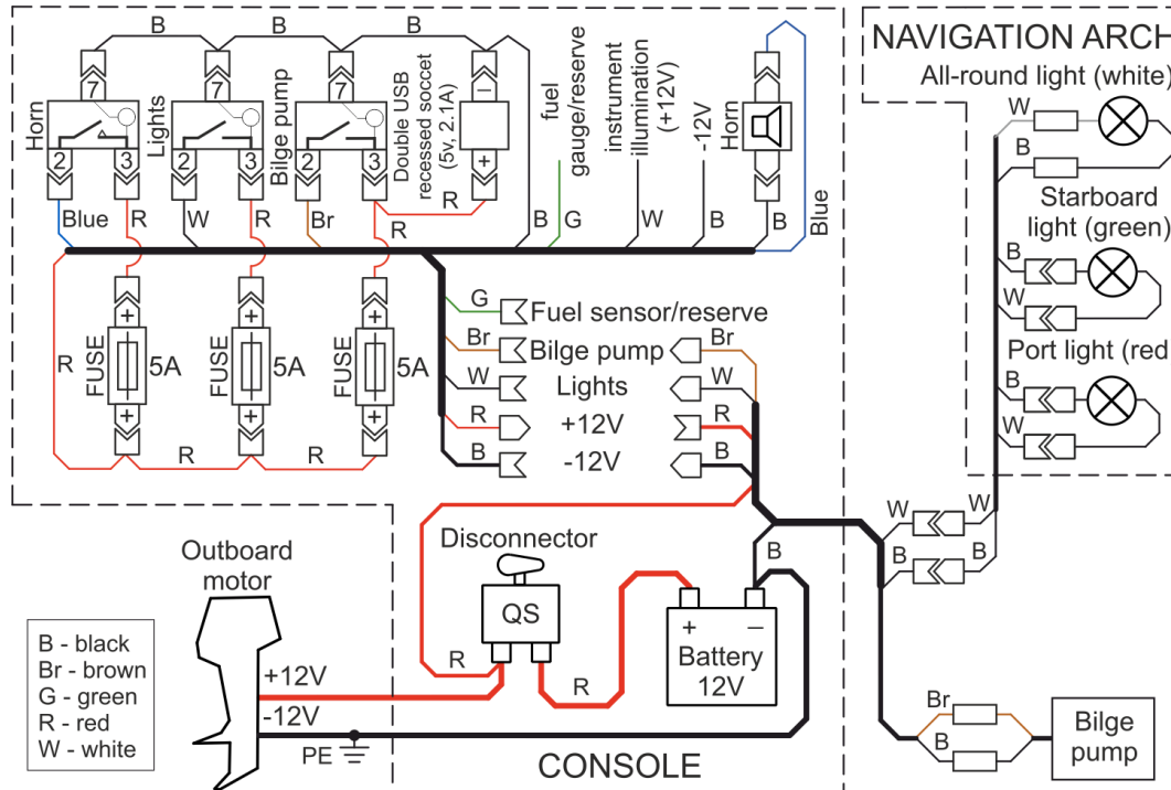
Fig. 57. Electrical schematic diagram with nav. lights on the navigation arch.
