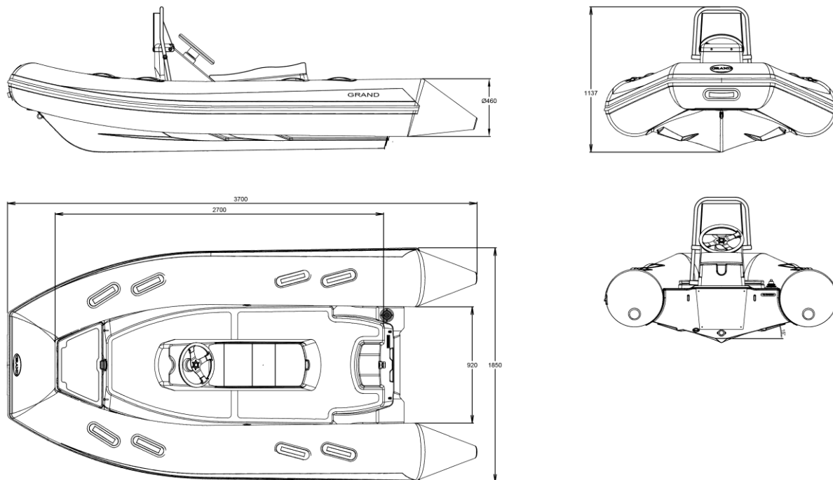
Fig. 44. General view of a boat S370NS.
