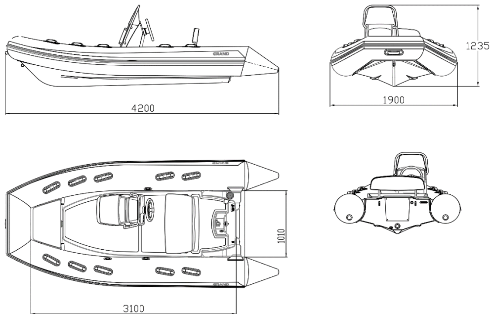
Fig. 53. General view of a boat S420NL.
