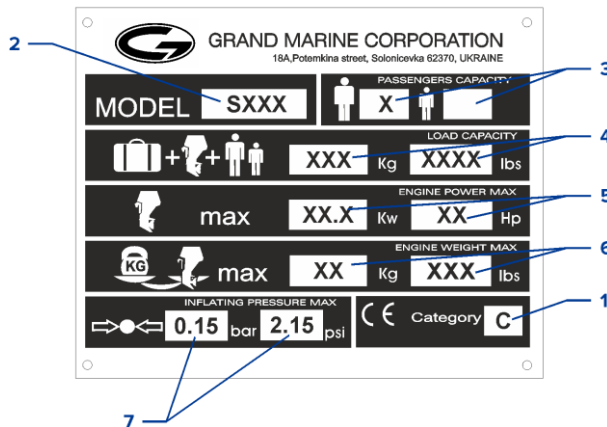
Fig. 5. Builder's plate.
