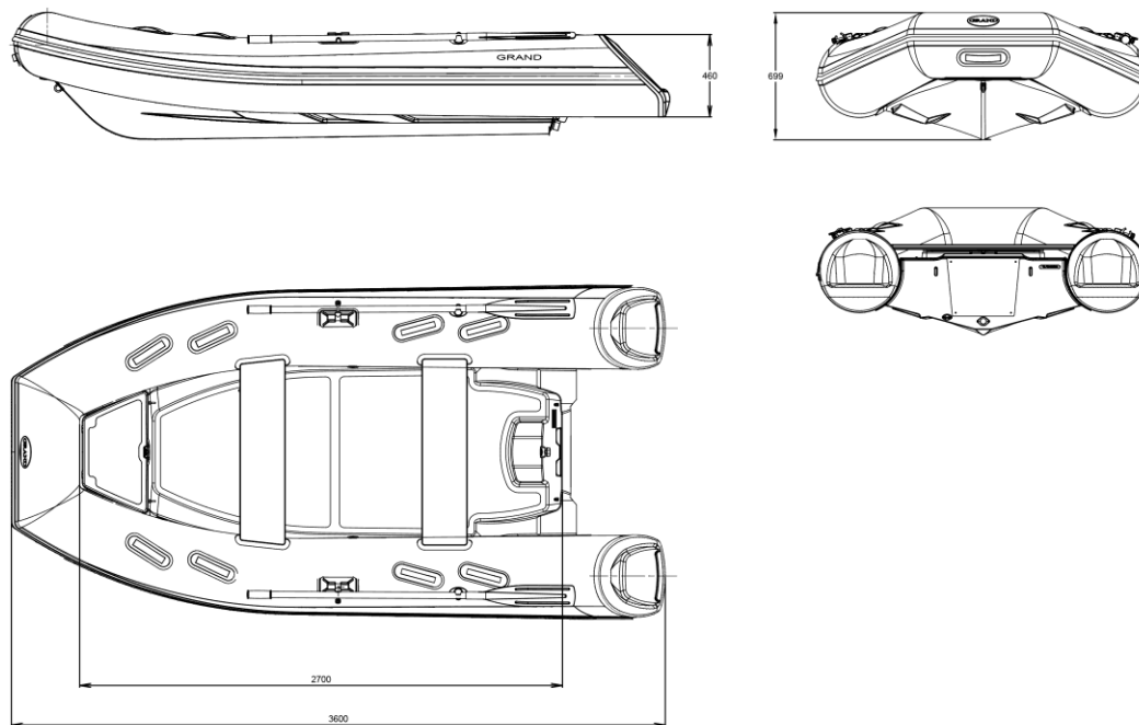
Fig. 43. General view of a boat S370NF.
