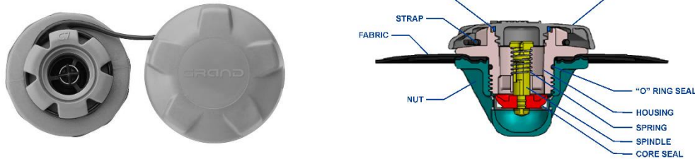
Fig. 10. Inflation valve (option 1).
