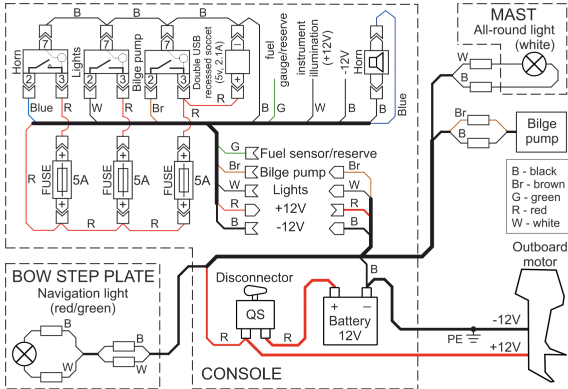
Fig. 58. Electrical schematic diagram with nav. lights on the bow step plate.
