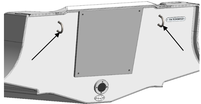
Fig. 26. Rear lifting eyes, 2 positions.
