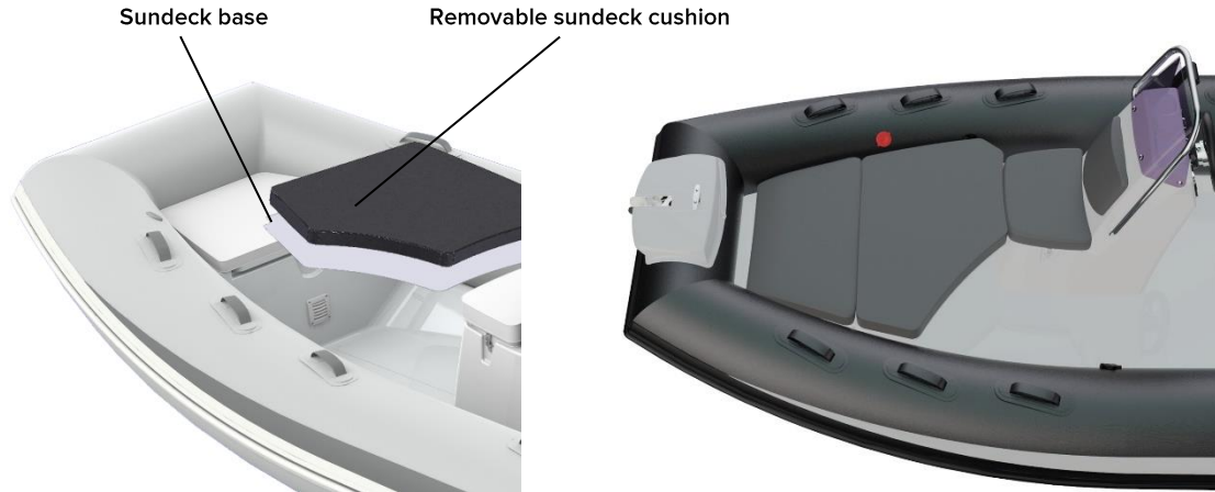
Fig. 32. Removable sundeck with cushion.
