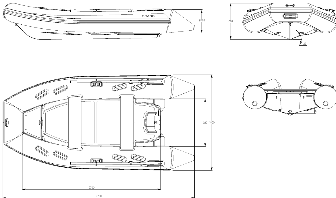
Fig. 42. General view of a boat S370N.
