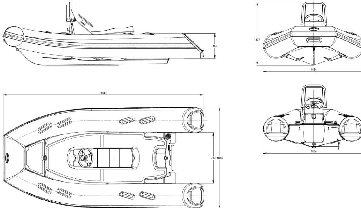
Fig. 45. General view of a boat S370NSF.
